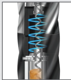
SpringAssist System
